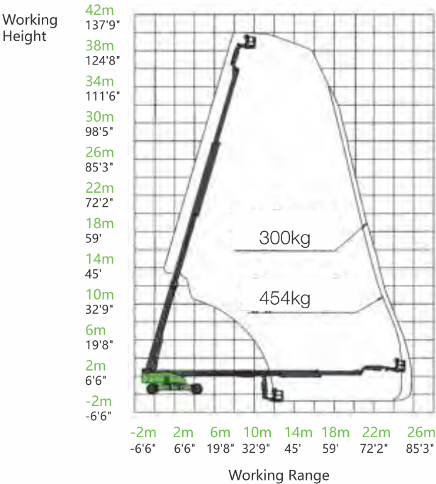
LT38JE-c Performance Curve
